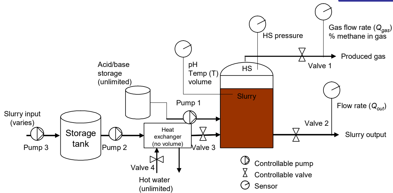
Figure 1. Biogas production process.
